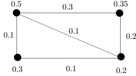
FIGURE 2. G_2 , A fuzzy graph with energy < 1
