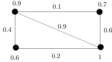
FIGURE 1. G_1 , A fuzzy graph
